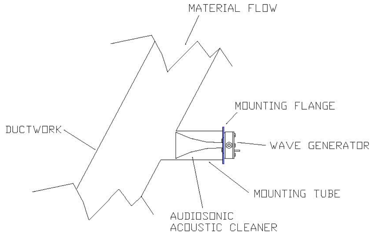
DRAWING N° PAS-G008
